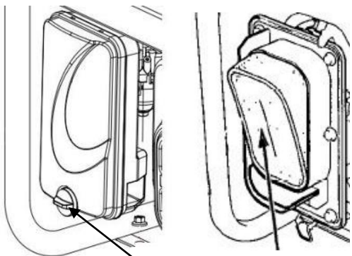
Turn Air Filter Cover Retainer and Remove Air Filter Cover and Element
